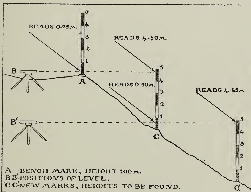
Fig. 5. The use of the Dumpy Level.
